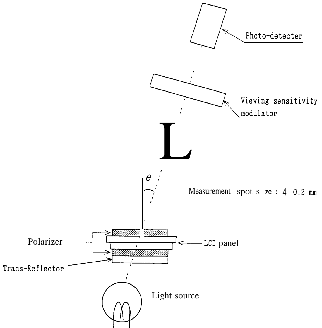
Fig.7-1 Optical Characteristics Test Method II (Transmissive mode)
