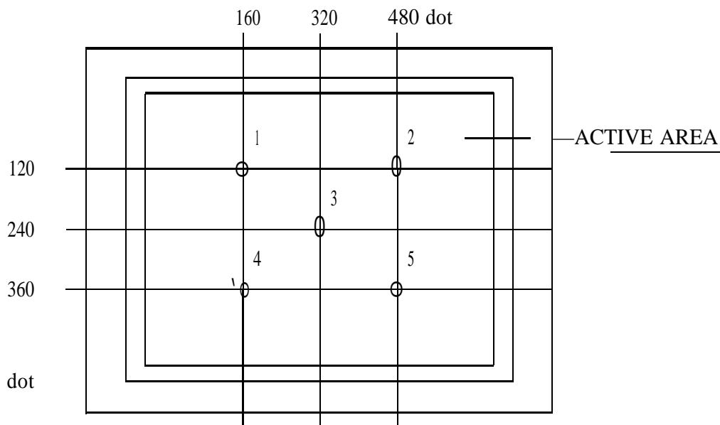
Fig.11 Measuring points(1~5)
